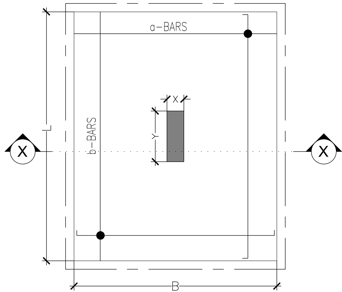
TYPICAL ISOLATED R.C. FOOTING
