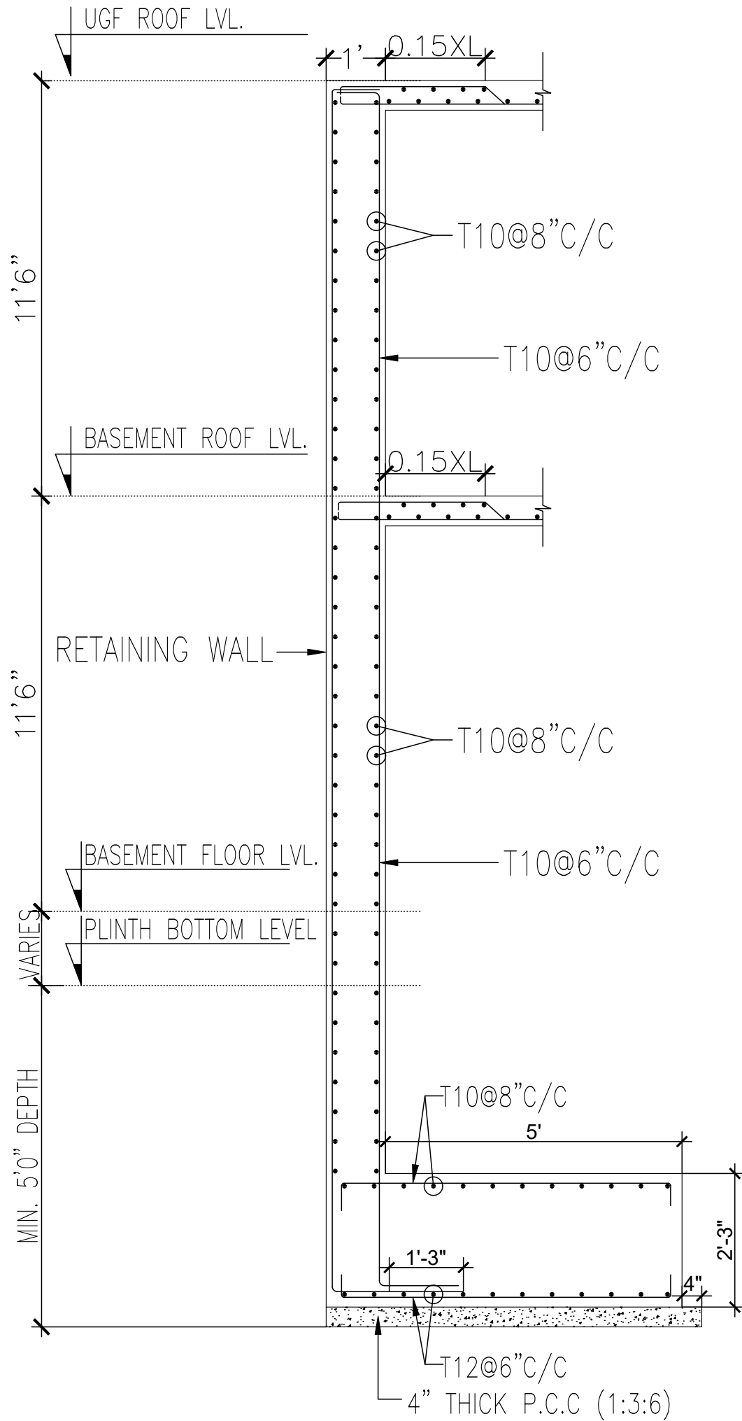
SECTION 01-01 RETAINING WALL-RW1
