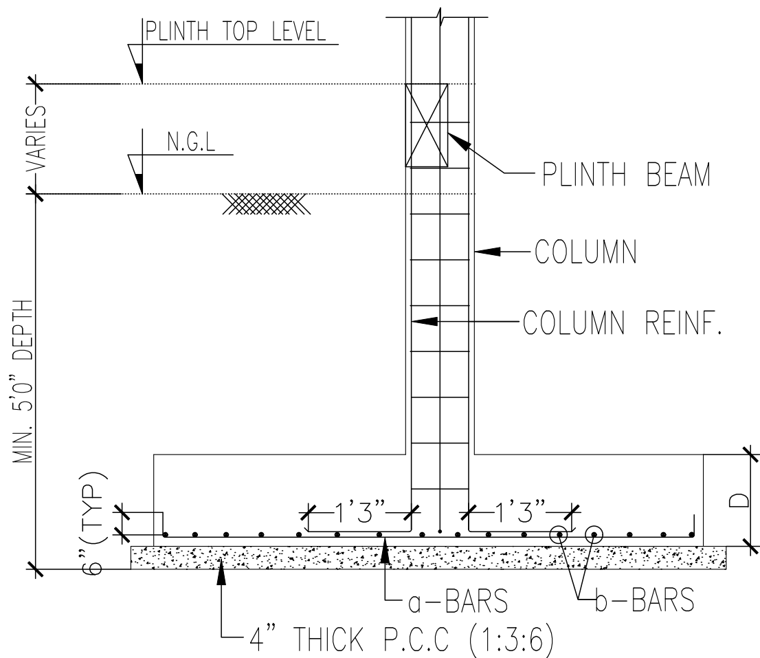
SECTION X-X
