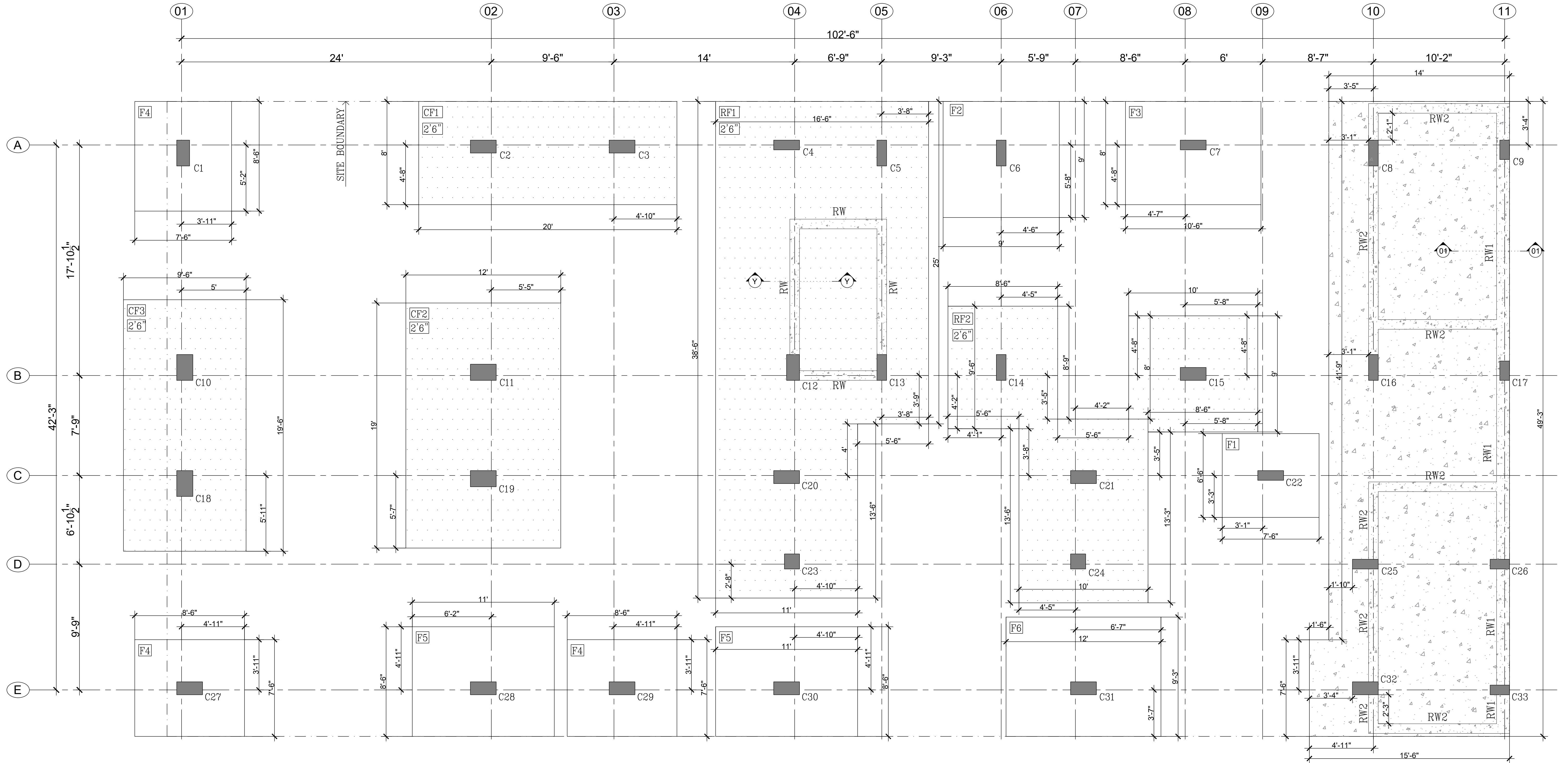
FOOTING LAYOUT
