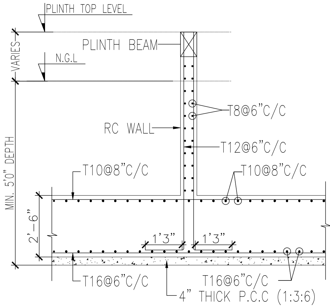
SECTION Y-Y RC WALL DETAILS
